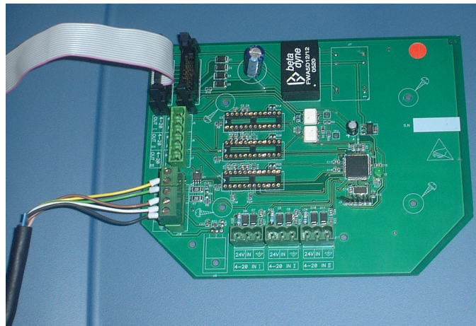
Figure 7: Connecting Turbidity Sensor to Turbidity Module
