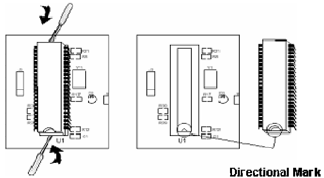
Figure 5: installing new chipset
