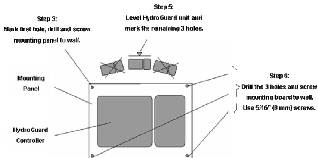
Figure 2: HydroGuard 702 Mounting Panel
