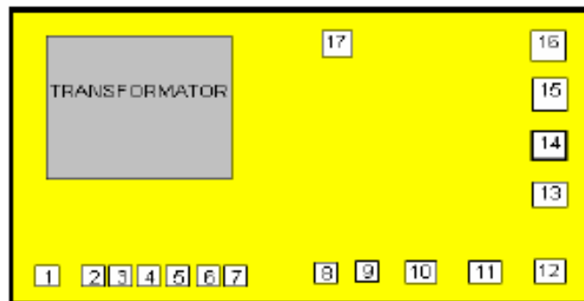
Figure 8: 4 to 20 mA Output Module Electrical connections
