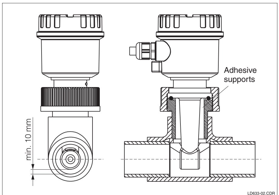
Pipe installation OLD 633 with PVC adhesive supports DN 40 (Accessories)
