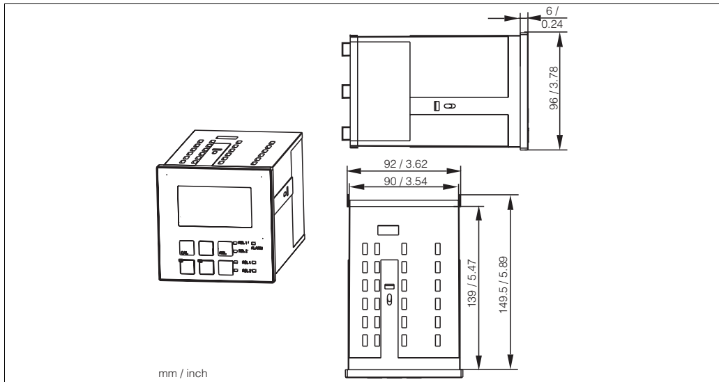
Fig. 4: Panel-mounted instrument
