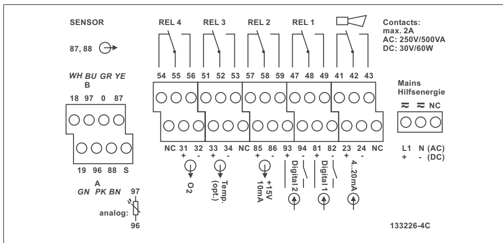
Fig. 20: Field instrument connection compartment sticker version WX/WS
