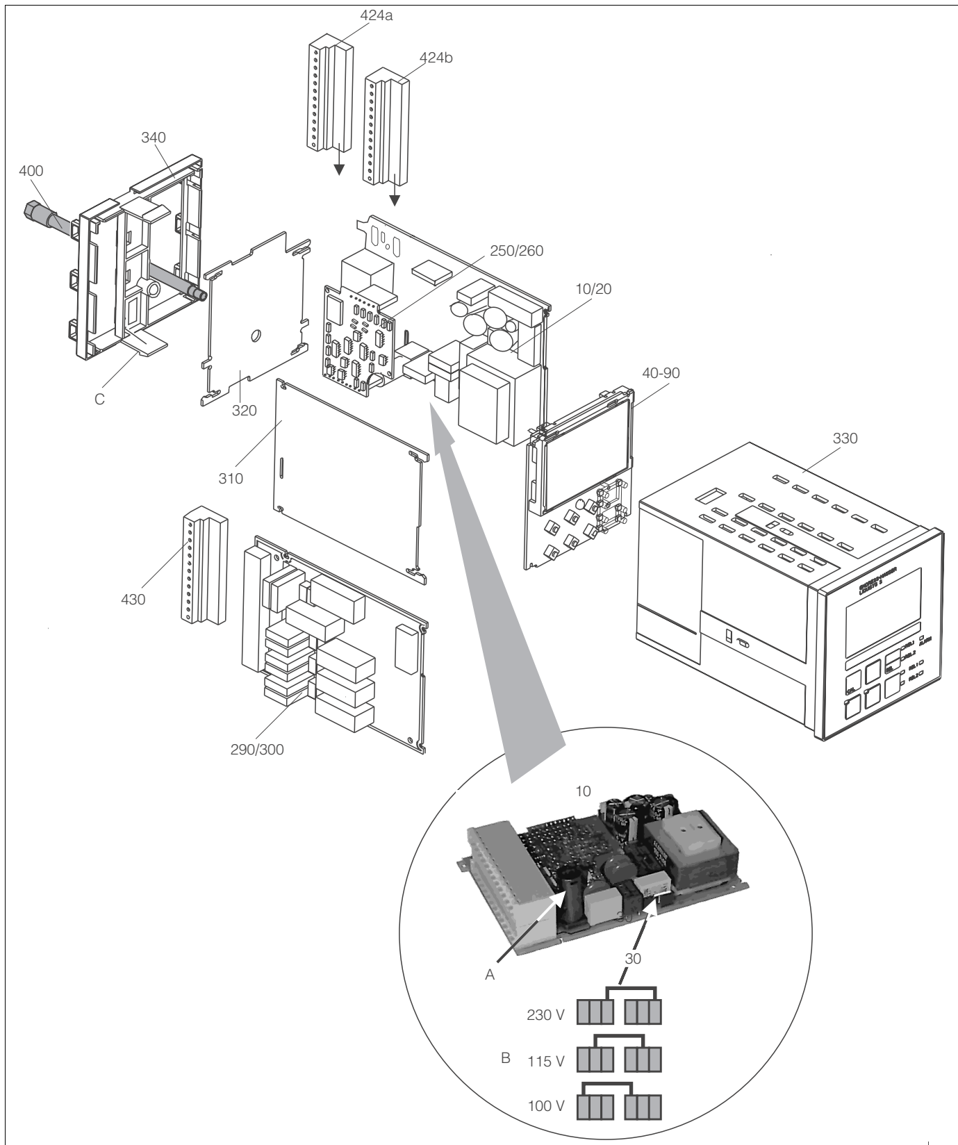
Fig. 44: Exploded drawing of panel mounted instrument
