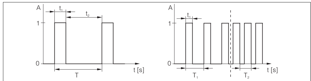
Fig. 37: Signal of a pulse-length modulated controller contact (left) and of a pulse-frequency modulated controller contact (right)
