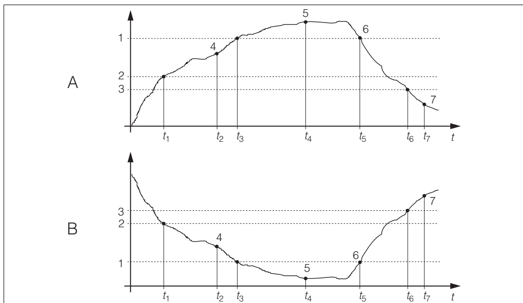
Fig. 34: Illustration of the alarm and limit value functions
