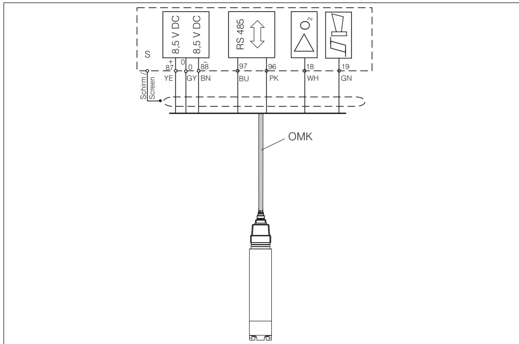
Fig. 22: Connection of OOS61 with OMK cable
