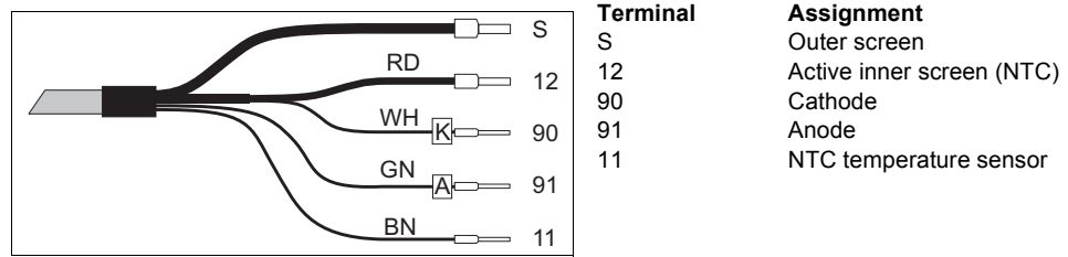
Fig. 12: Measuring cable CMK or OYK71
