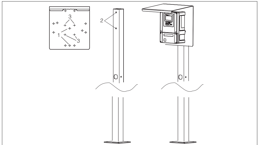
Fig. 7: Mounting field device with universal posts and weather protection cover
