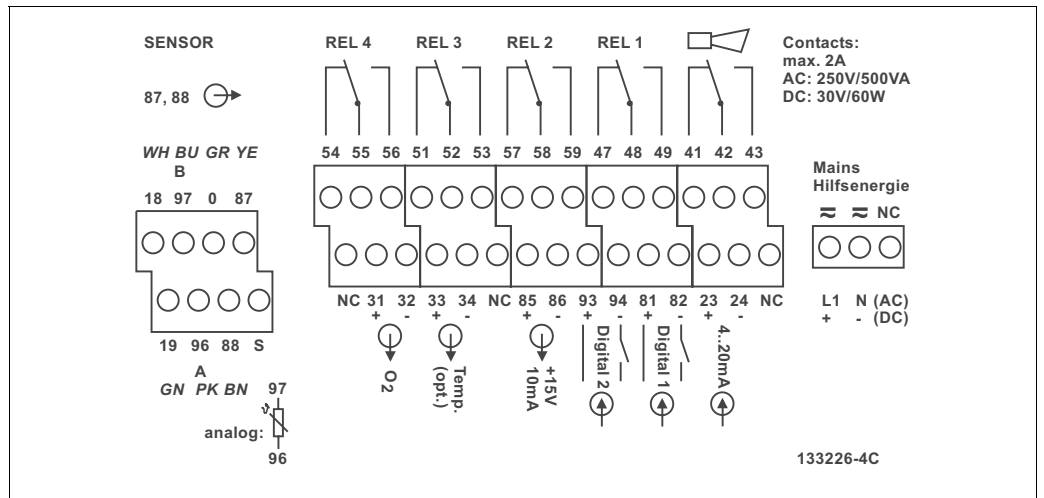
Fig. 15: Field instrument connection compartment sticker version WX/WS
