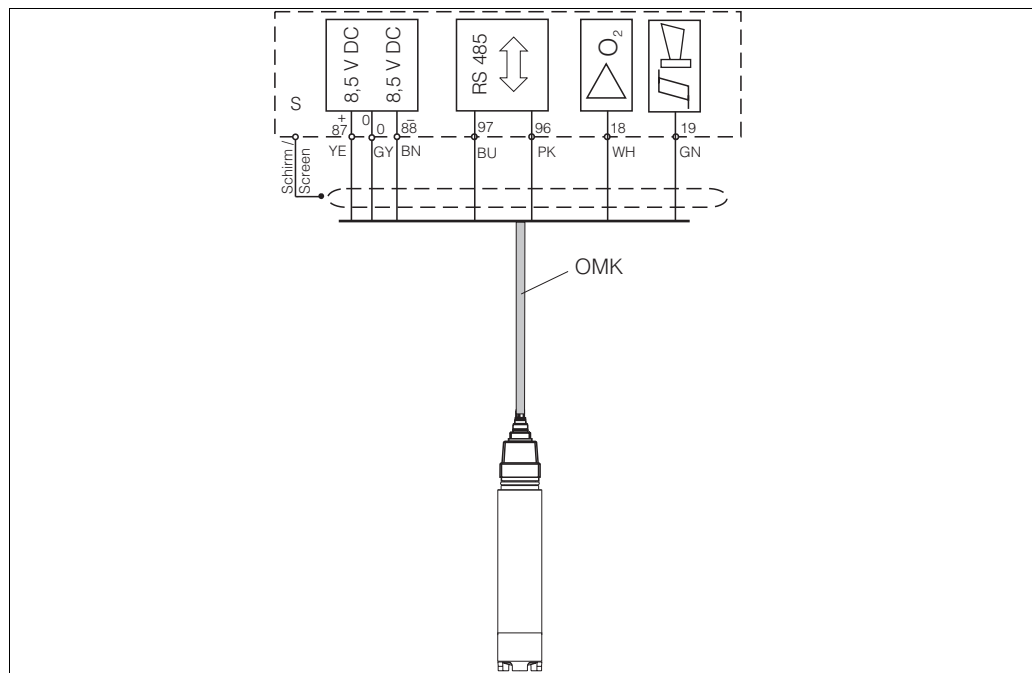
Fig. 18: Connection of OOS31/71 with OMK cable
