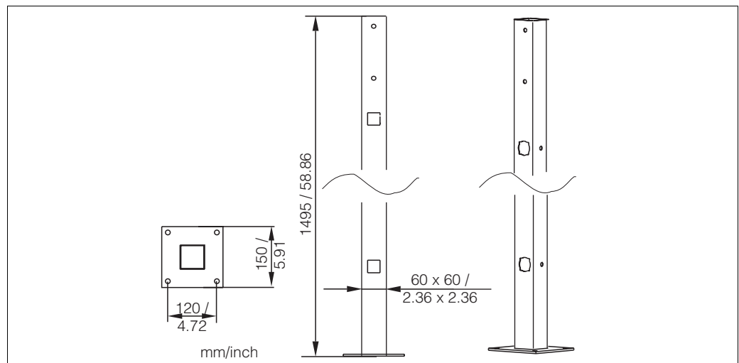
Fig. 42: Square post OYY102
