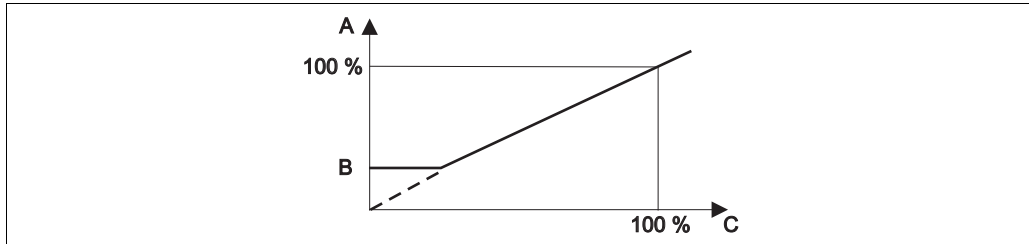
Fig. 35: Control characteristic PID controller with basic load dosing
