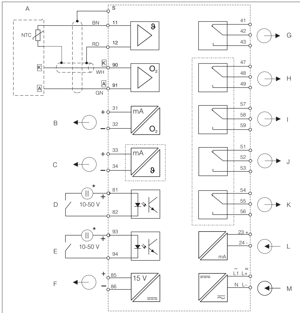
Fig. 9: Electrical connection of the transmitter in version DX or DS
