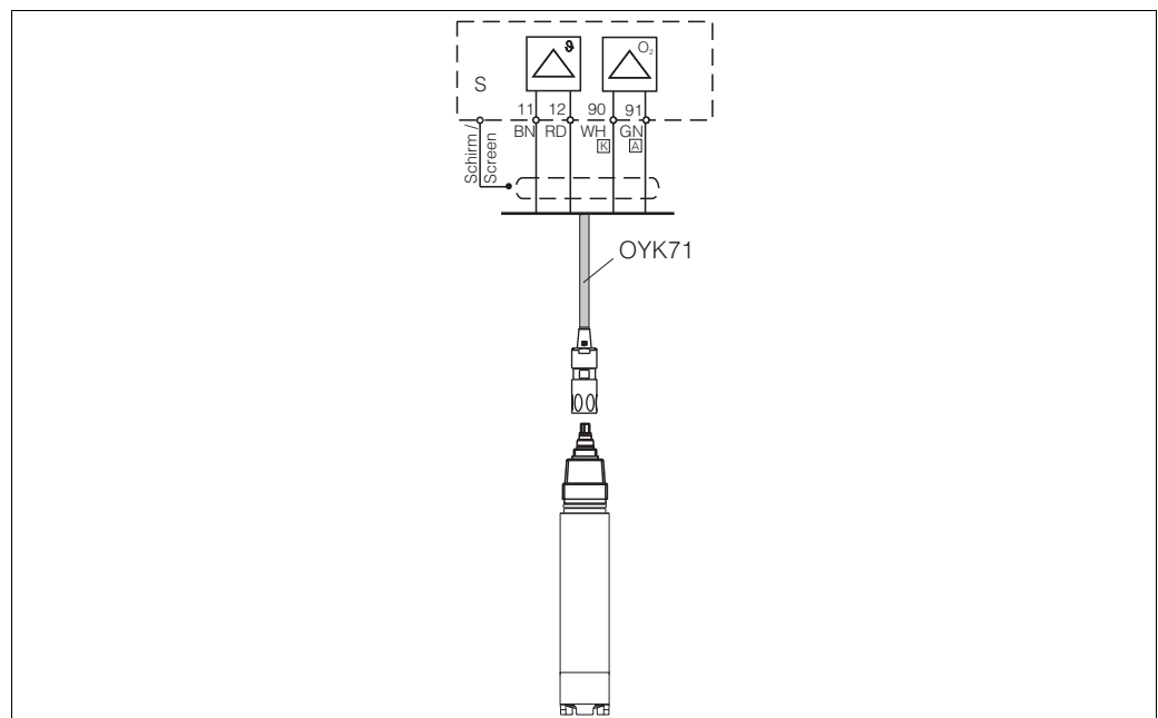
Fig. 13: Connection of OOS41 with OYK71 cable
