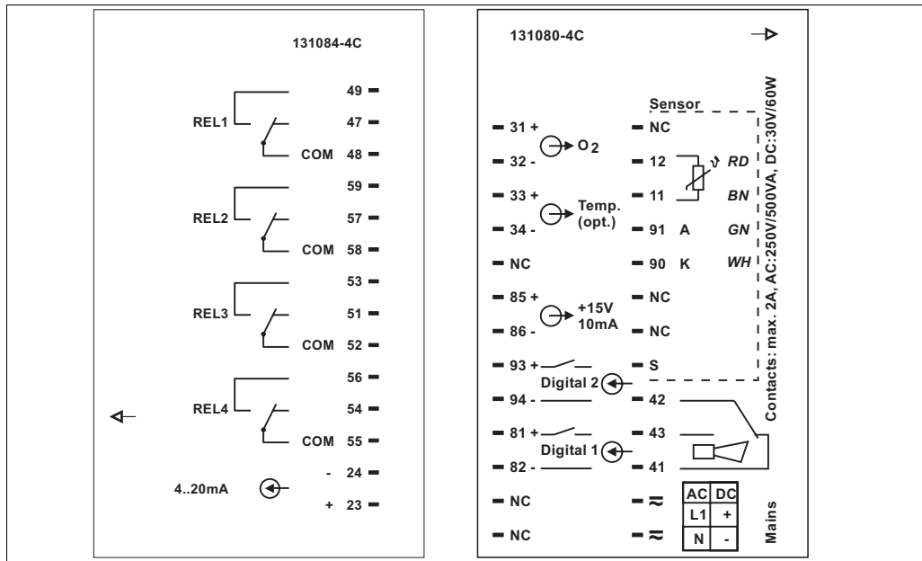
Fig. 11: Panel mounted instrument connection sticker
