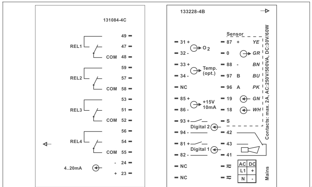
Fig. 16: Panel mounted instrument connection sticker
