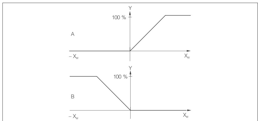
Fig. 38: Control characteristic of a proportional controller with direct and inverse control action
