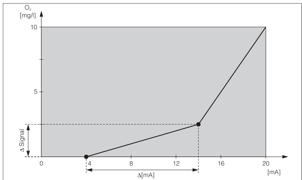
Fig. 33: User-defined current output characteristic (example)
