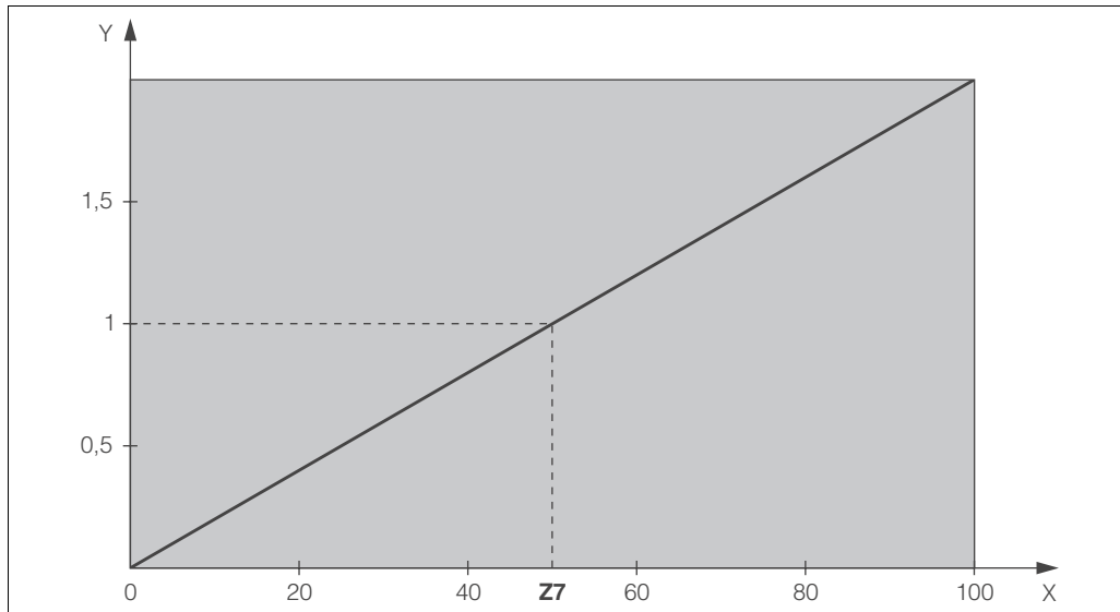
Fig. 32: Multiplying feedforward control
