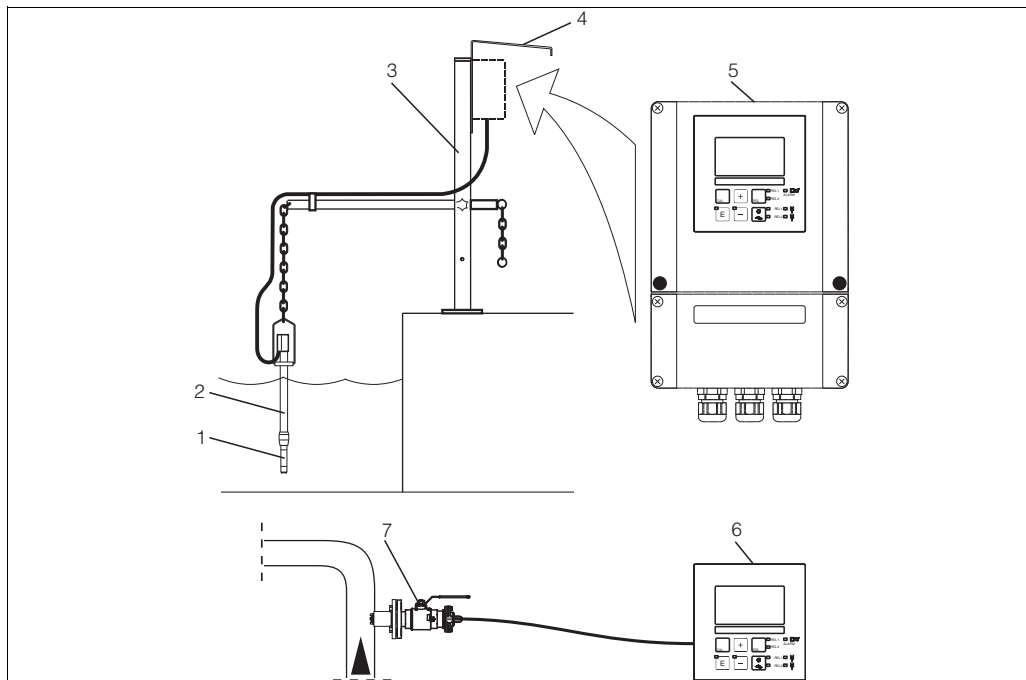
Fig. 1: Complete measuring system OOM223/253
